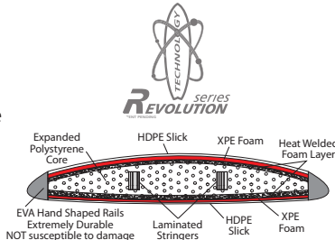
Cross Section Construction
